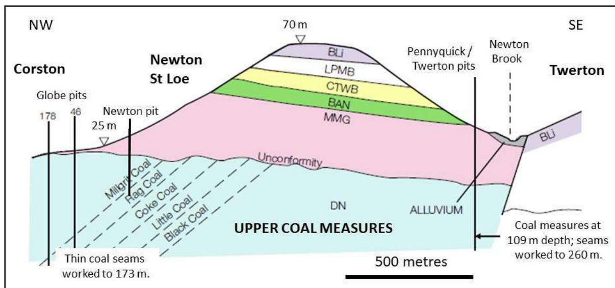
Figure 2. Cross-section from Twerton to Corston showing the geology and the location of the coal mines. Key: BLI = Blue Lias, LPMB+CTWB+BAN = Rhaetic, MMG = Mercia Mudstone, DN = Downend Formation (modified from BANES 2010 Slope geological instability and undermining study, Twerton and Odd Down. Report 028/10, Ove Arup & Partners Ltd, Bristol.).
