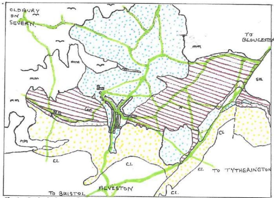
Fig. 1 – Geological map of Thornbury area (from BGS Bristol District Special Sheet 1962)
