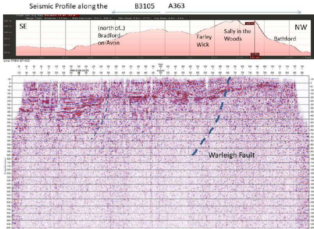
Figure 5. Seismic Profile PPBW-87-003
