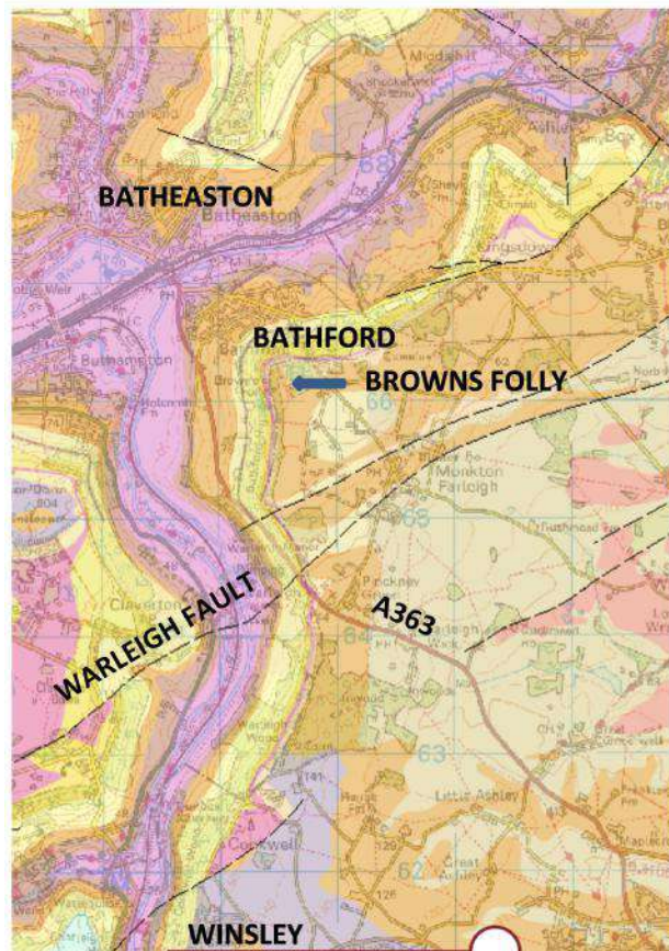
Figure 2 i-geology map courtesy of BGS
