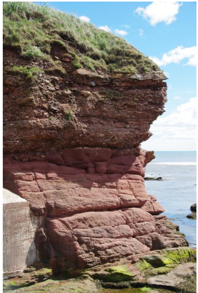
Fig. 3: Whiting Ness unconformity
