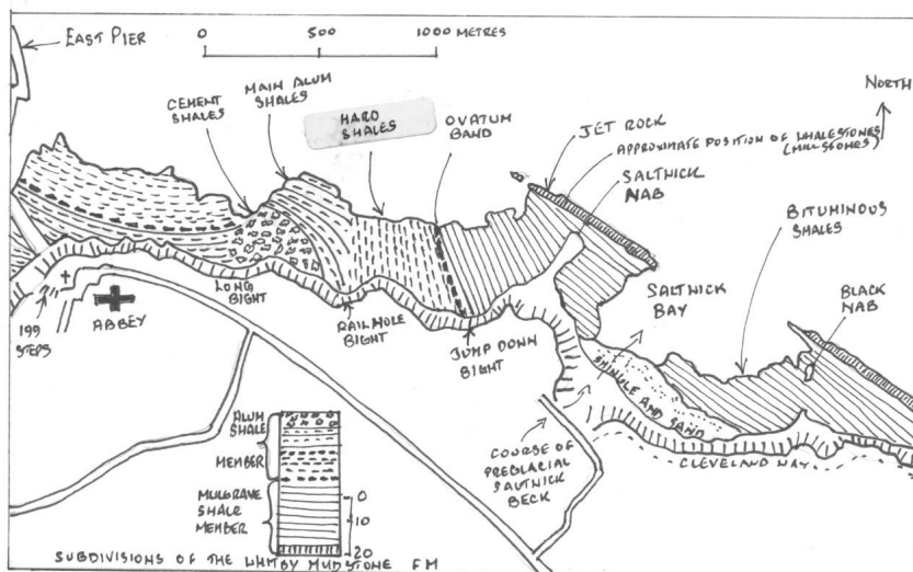
Map to show the geology from Saltwick to Whitby
