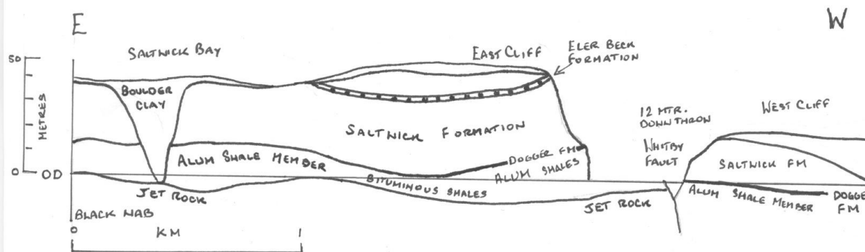
E-W section from Saltwick Bay to West Cliff
